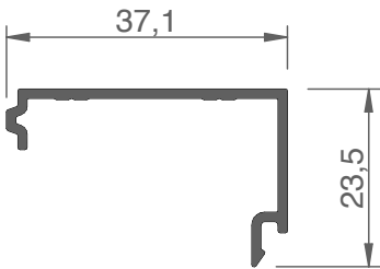
FWP10008 junquillo celosia
