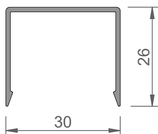
FWP10008 junquillo celosia
